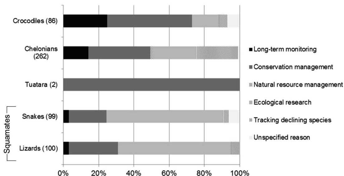
FIG. 4. Data sources publishing time-series data for reptiles, by major reptile group. There were no population time series for amphisbaenians in the LPD.
