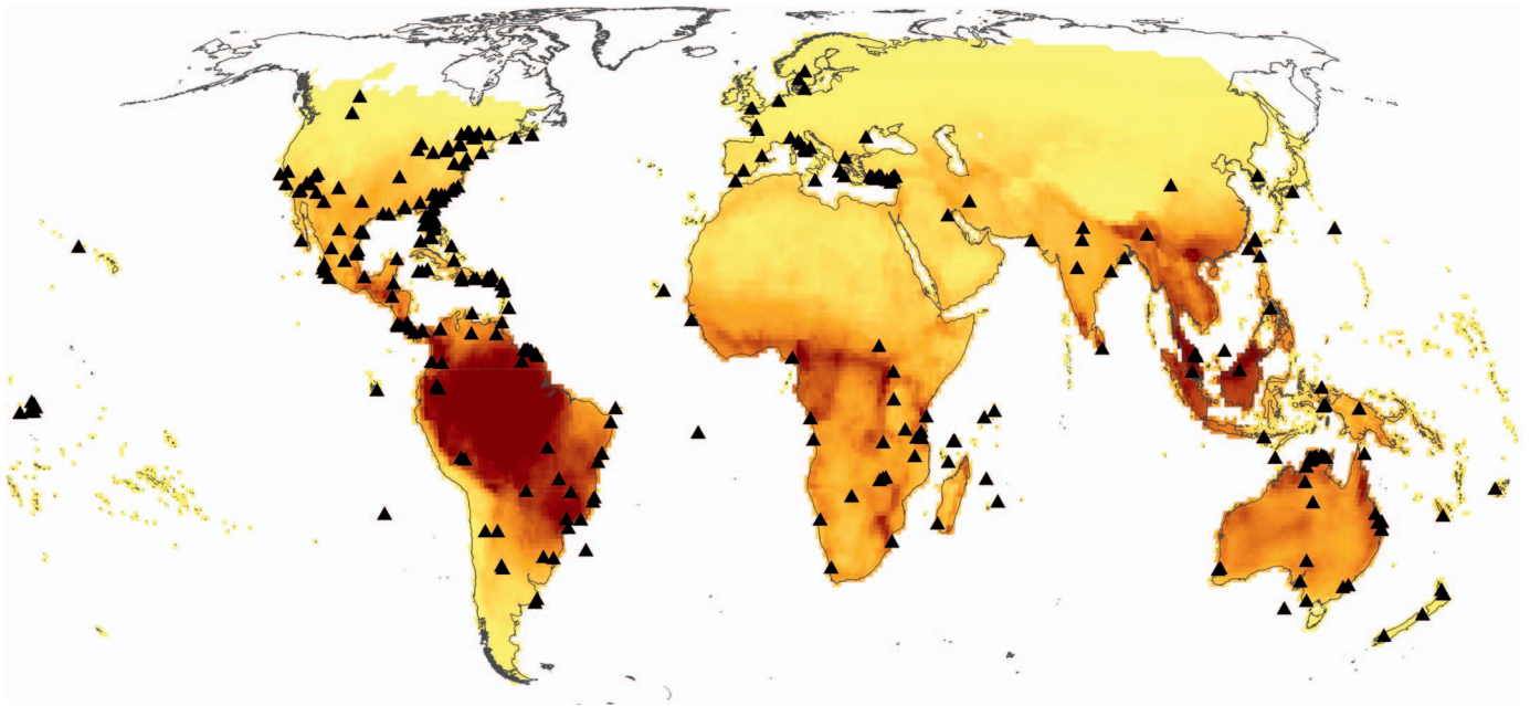
FIG. 3. Spatial distribution of population time-series data (triangles) for reptiles with data held in the LPD, superimposed on a global map of reptile species richness at 1-degree spatial resolution (Roll et al., 2017). Darker cells have higher species richness (maximum richness is 204 species per cell). Separate maps by taxon groups are presented in Figure S3.
